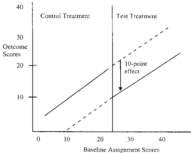
Fig. 1 Regression-discontinuity design with a 10-point treatment effect.
