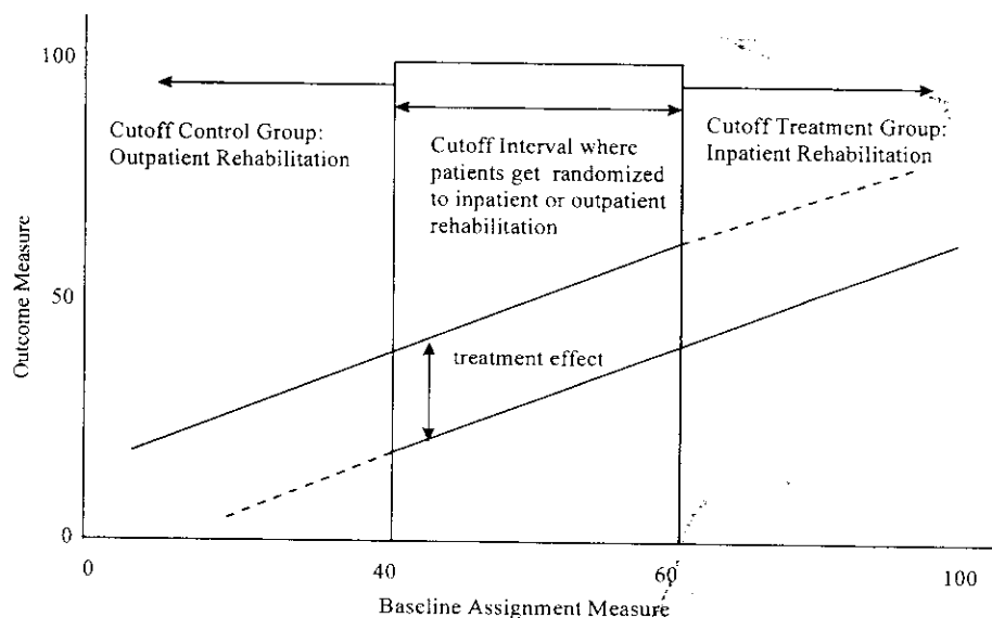
Fig. 3 Illustration of a combined randomized and regression-discontinuity design.
