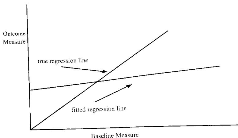
Fig. 2 Regression to the mean: randomized design and regression-discontinuity design.
